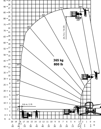
Rotation on lowered stabilisers with 365 kg platform EN 280
