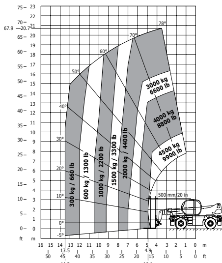
Rotation on lowered stabilisers with 5000 kg winch EN 1459
