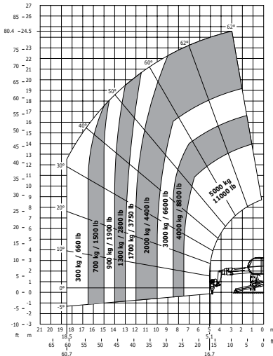
Rotation on lowered stabilisers Positive 3D platform EN 280
