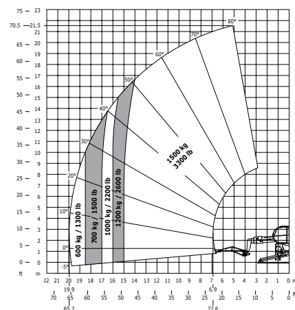
Rotation on lowered stabilisers with 1500 kg jib EN 1459
