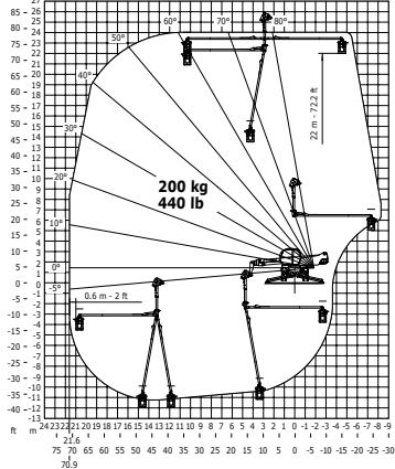
Rotation on lowered stabilisers Negative 3D platform EN 280
