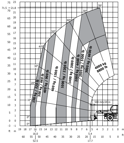
Front loader on tyres with forks EN 1459
