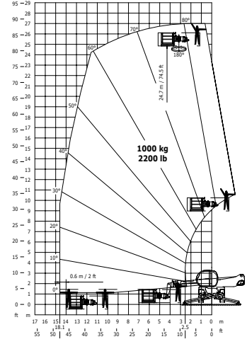
Rotation on lowered stabilisers with 1000 kg platform EN 280
