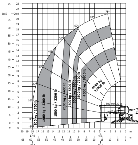
Rotation on lowered stabilisers with forks
