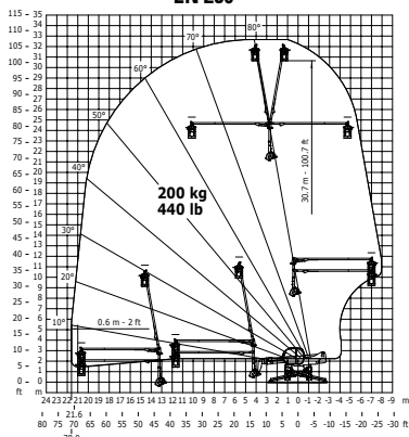
Rotation on lowered stabilisers Positive 3D platform EN 280
