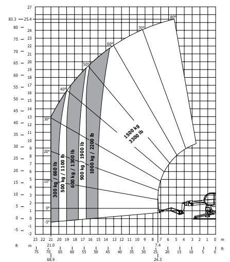
Rotation on lowered stabilisers with 1500 kg jib EN 1459
