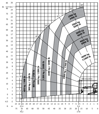
Rotation on lowered stabilisers with forks EN 1459
