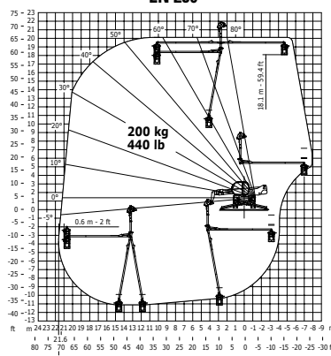
Rotation on lowered stabilisers Negative 3D platform EN 280
